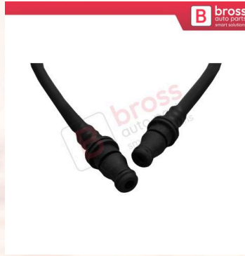
BHC634 Engine Coolant Recovery Tank Breather Pipe 2115010625 for Mercedes E320 E350 E280 Length 545 mm
