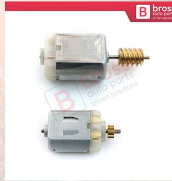
BGE661+BGE662 Door Lock 12V DC Motor Gear Set For Ford Volvo Land Range Rover Jaguar Mazda
