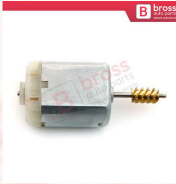
BGE671 Door Central Control Lock Actuator FC280 Motor Gear 20 mm Shaft for Peugeot Citroen
