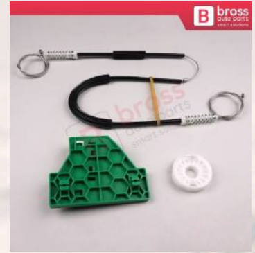
BWR273 Window Regulator Repair Kit Rear Left Door for Audi A4 B6 8E2 8E5 B7 8EC 8ED Seat Exeo 3R 4/5 Door 8E0839461
