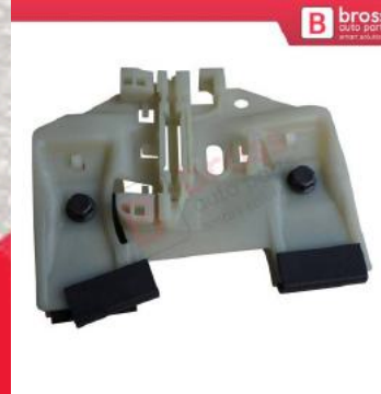
BWR5364 Window Regulator Repair Clips Right A9067200146 for Mercedes Sprinter MK2 VW Crafter MK1
