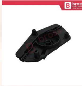
BWR5159 Window Regulator Motor Cover Front Left Door for Citroen C4 Picasso 2006-On
