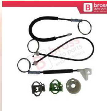
BWR233 Window Regulator Repair Kit Front Right Door for VW Polo Classic 6V2 6KV2 Variant 6V5 Caddy MK2 9K9 9U 6K4837402P
