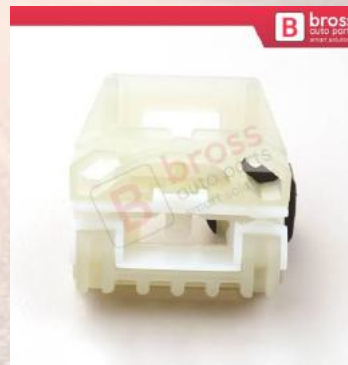
BWR525 Window Regulator Clip Front Left Door for VW New Beetle Seat Ibiza 1999-2008 Seat Leon MK1 Seat Toledo MK2 Skoda Fabia 1999-2007
