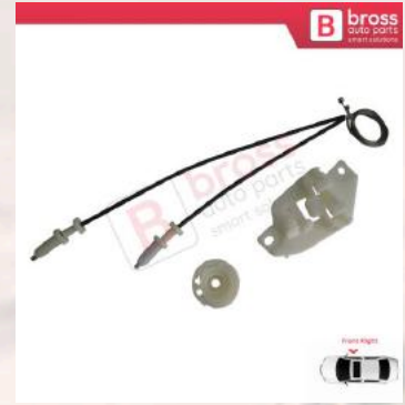
BWR5244 Window Regulator Repair Set Front Right 824024A000 for Hyundai H 1 Starex MK1
