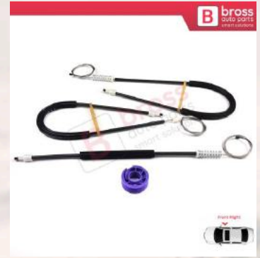
BWR515 Power Window Regulator Repair Set Front Right Door for Seat Toledo MK3 5P2 2004-2009 Altea 5P1 XL 5P5 5P8 5P0837462
