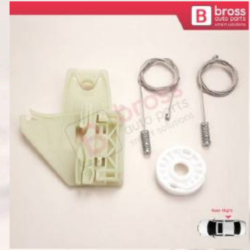
BWR5077 Power Window Regulator Repair Set Rear Right for Skoda Octavia MK2 A5 1Z3 1Z5 2004-2013 4/5-Door 1Z0839656
